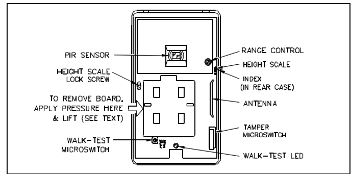
Fig. 2. GEM-DT, front cover removed.
